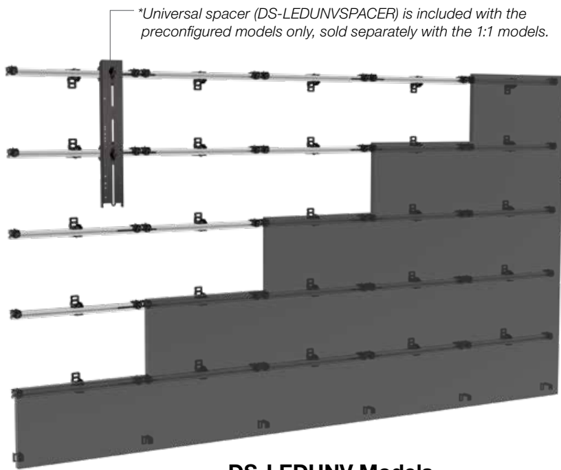
DS-LEDUNV Models
