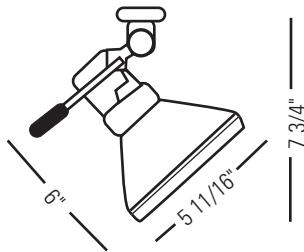
PAR38 Bezel with Par-Tech® Incandescent/halogen Fixture 8202
