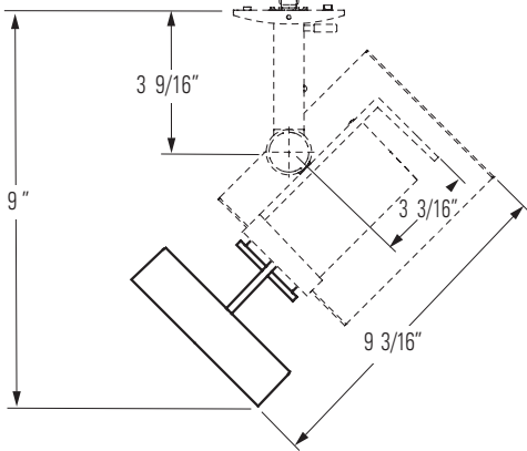
RING PAR20 WITH METALLICS™ ELECTRONIC METAL HALIDE FIXTURES 8704E, 8705E, & 28705E (PROSPEC)
