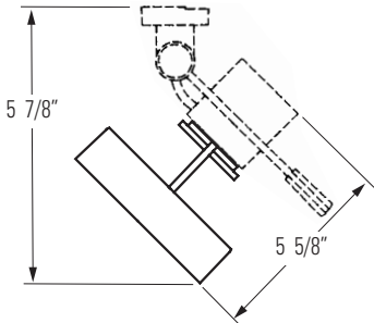
RING PAR30 WITH PAR-TECH® INCANDESCENT/HALOGEN FIXTURE 8202
