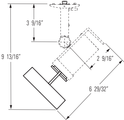
RING PAR20 WITH METALLICS™ INCANDESCENT/HALOGEN FIXTURES 8701 & 28701 (PROSPEC)
