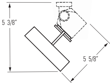
RING PAR30 WITH PAR-TECH® INCANDESCENT/HALOGEN FIXTURE 8201
