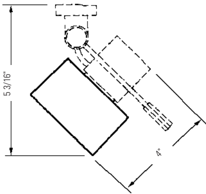
CYLINDER 20 WITH HINGED ADAPTER
